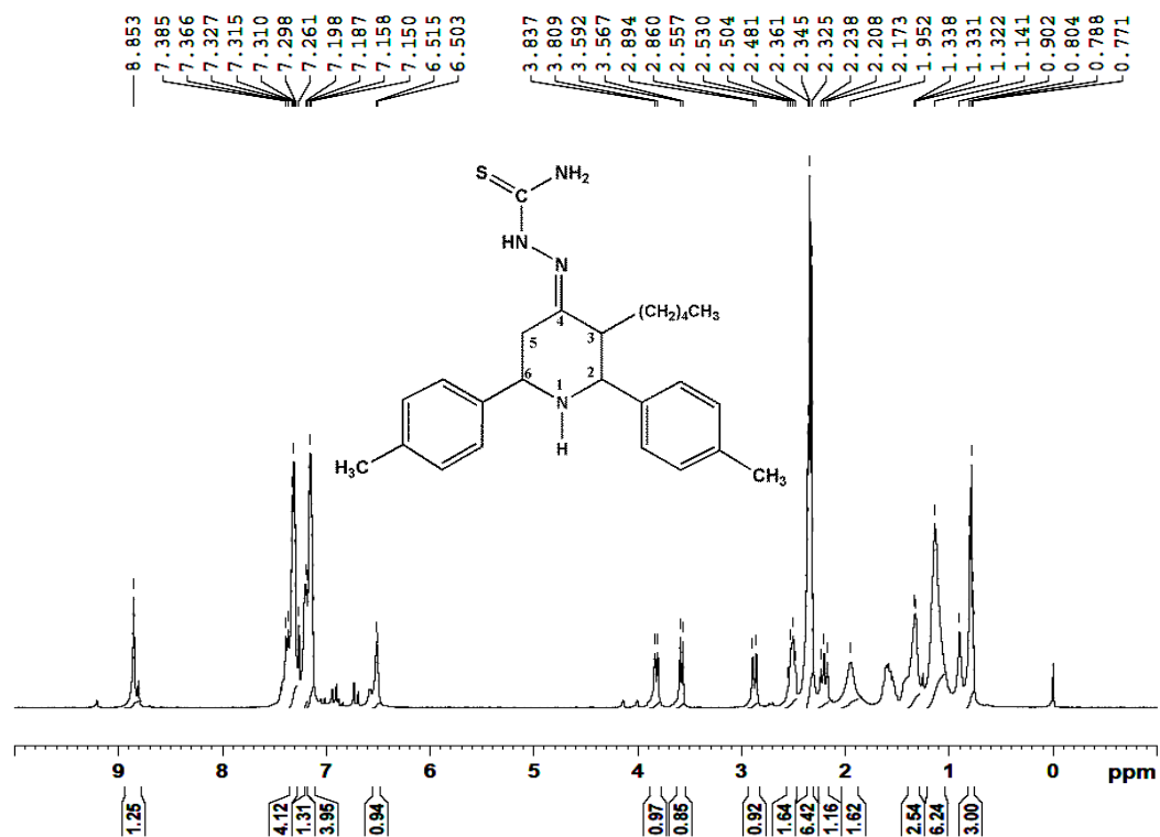
Figure 23. 1 H NMR Spectrum of 7 in CDCl 3
