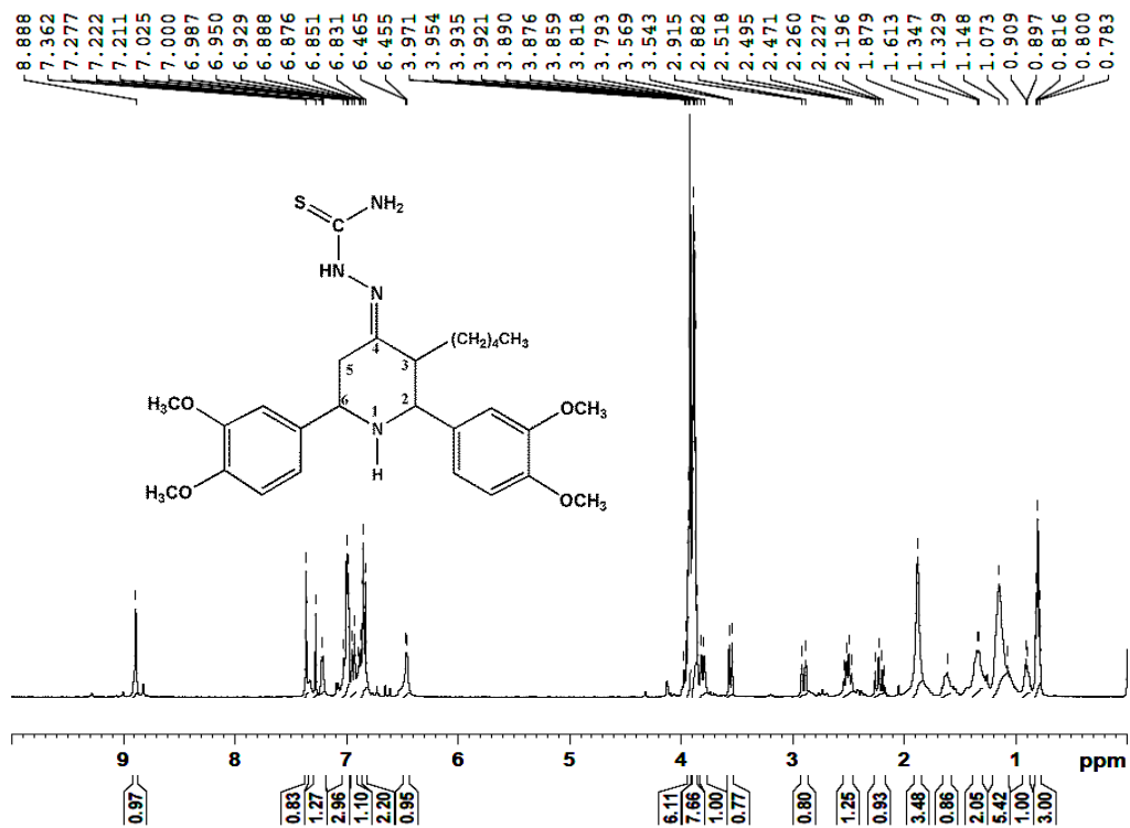
Figure 20. 1 H NMR Spectrum of 6 in CDCl 3
