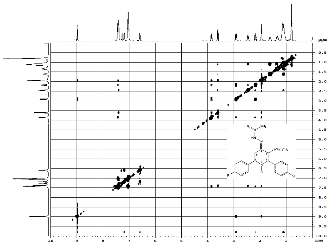
Figure 9. NOESY spectrum of 2 in \text{CDCl}_3
