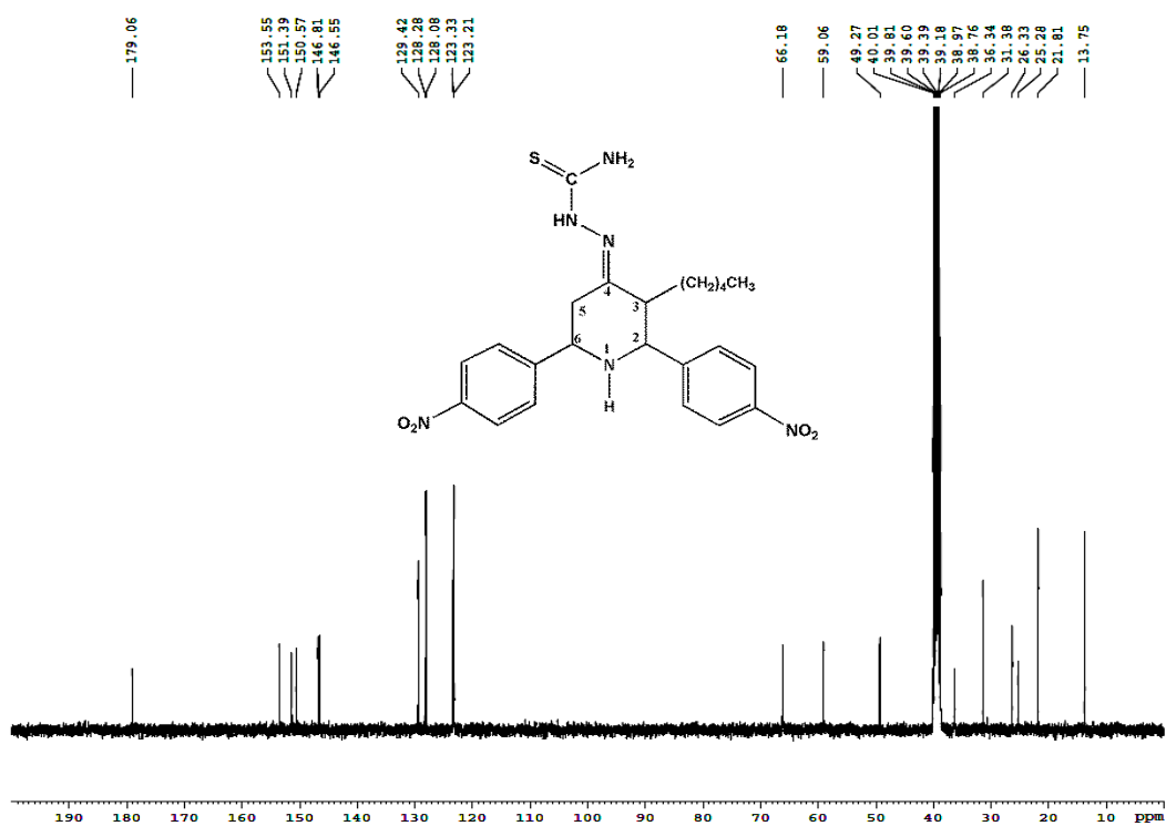
Figure 15. 13 C NMR Spectrum of 4 in DMSO
