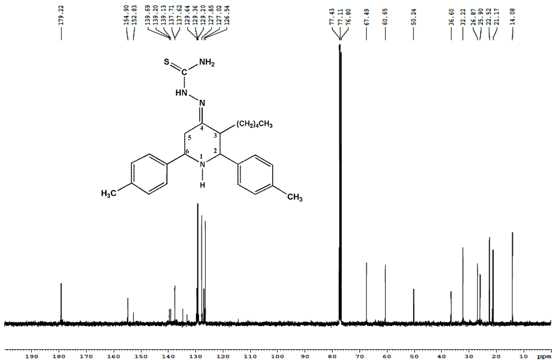
Figure 24. 13 C NMR Spectrum of 7 in CDCl 3
