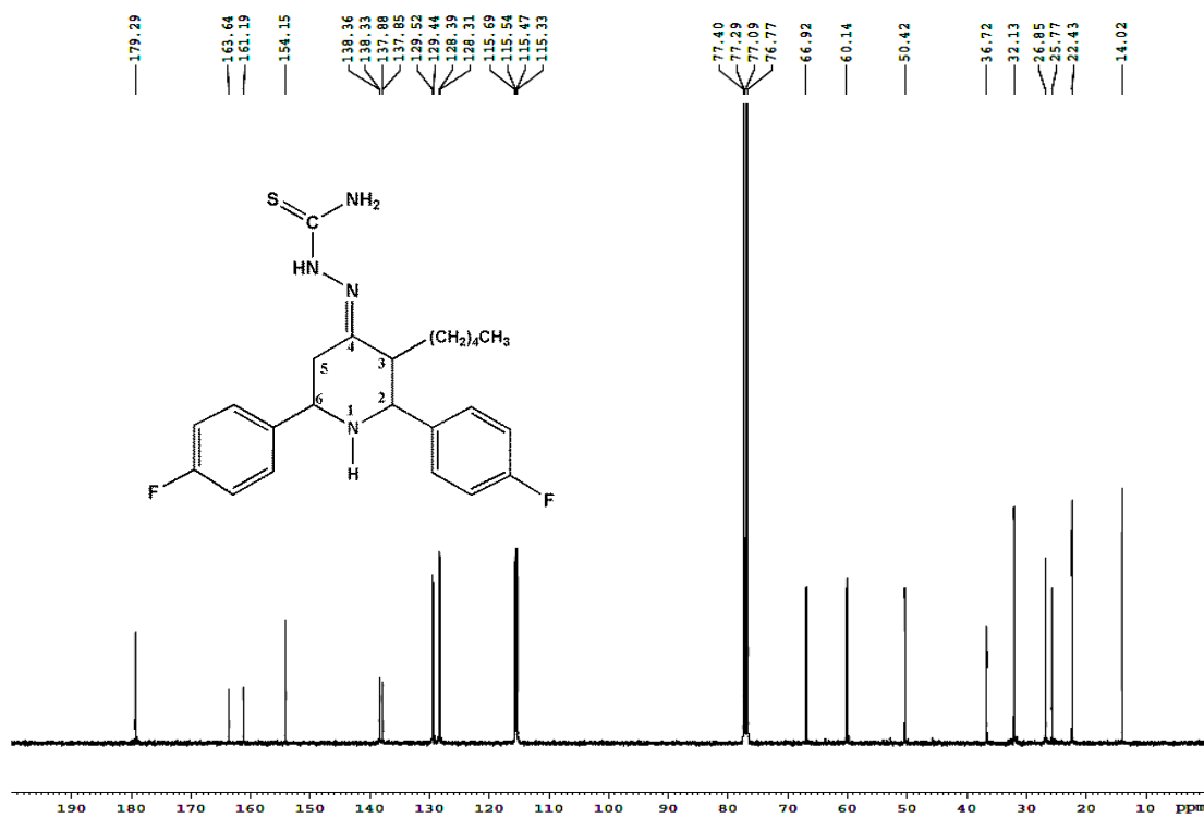
Figure 5. ^{13}\text{C} NMR Spectrum of 2 in \text{CDCl}_3
