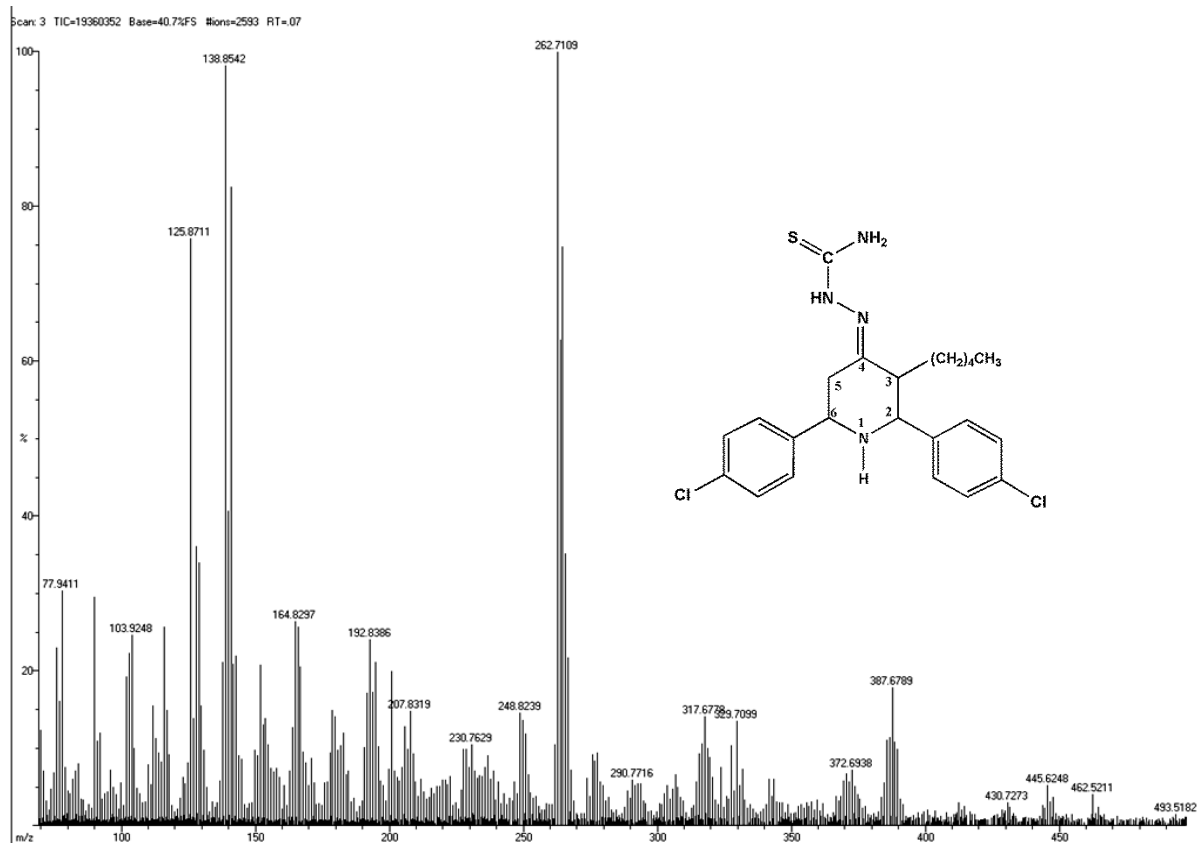
Figure 13. Mass Spectrum of 3
