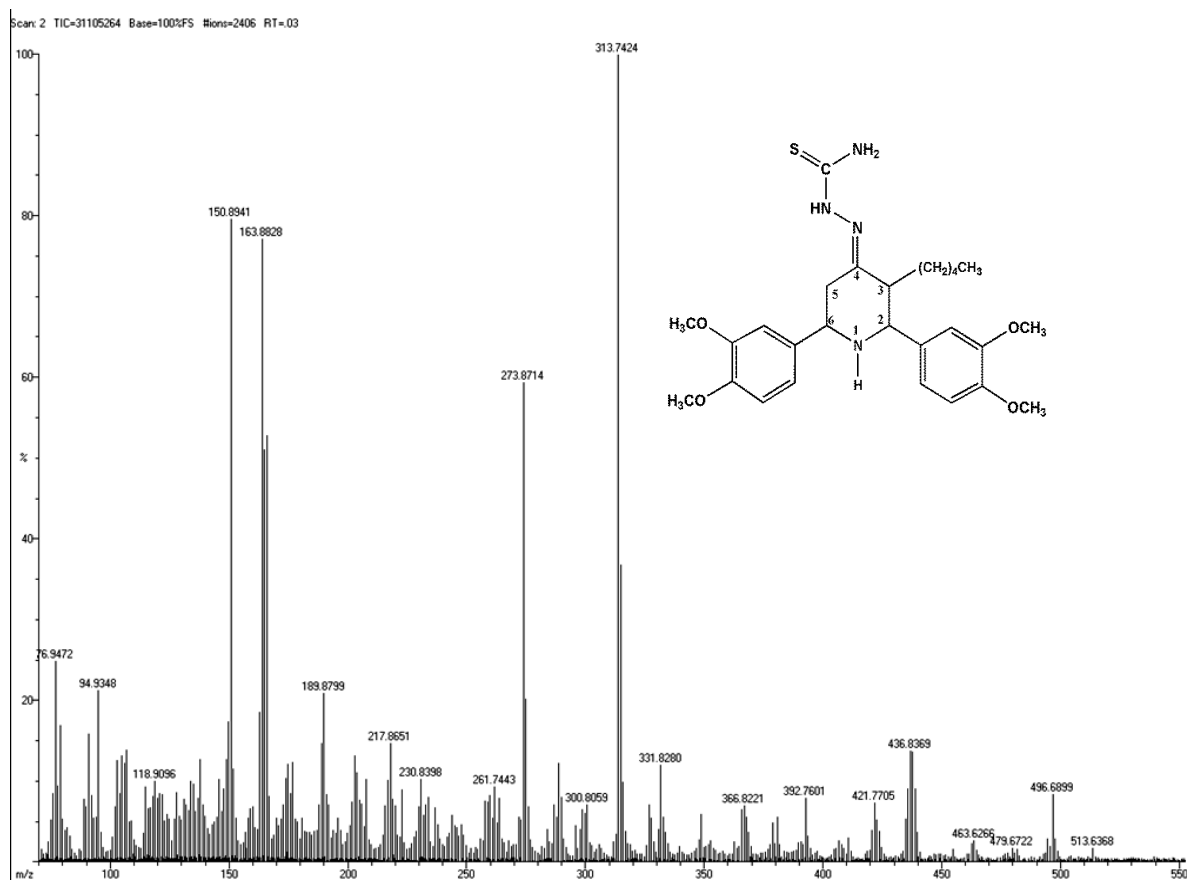
Figure 22. Mass Spectrum of 6
