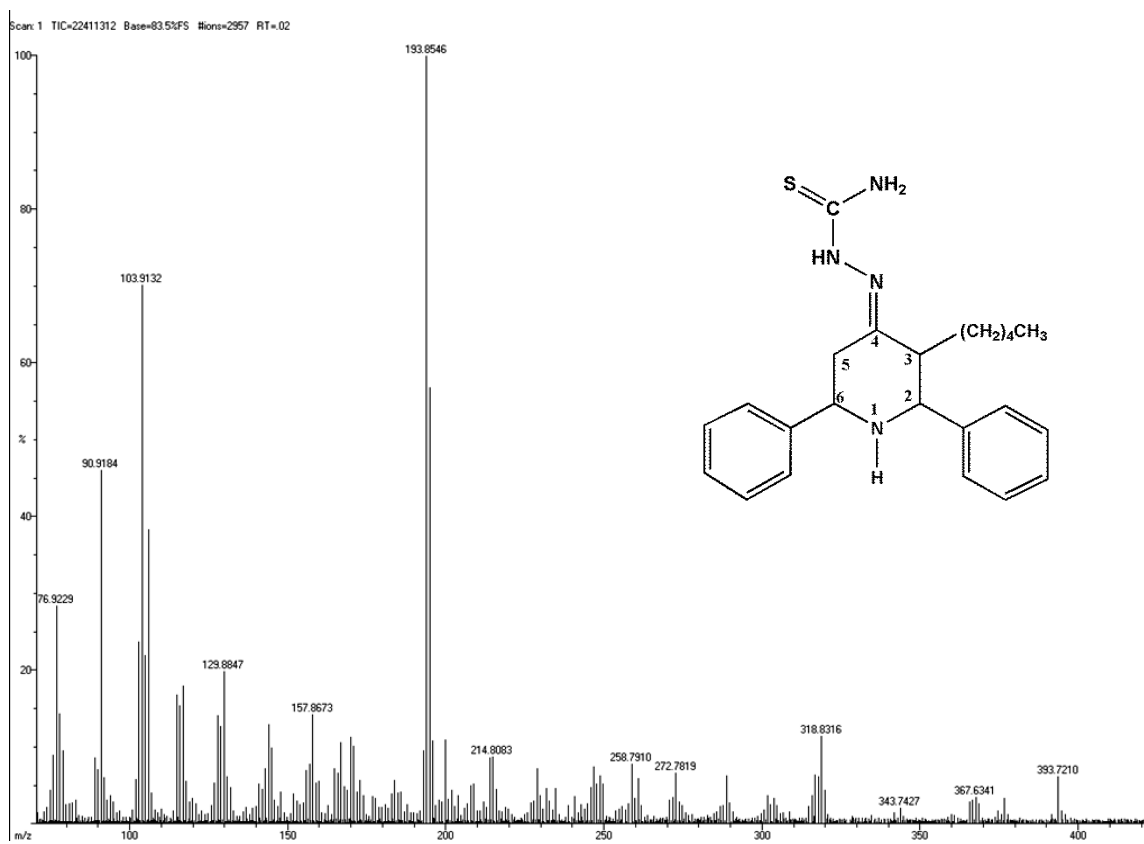
Figure 3. Mass Spectrum of 1
