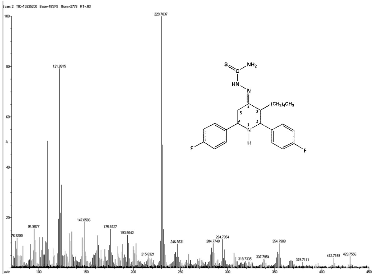
Figure 10. Mass Spectrum of 2
