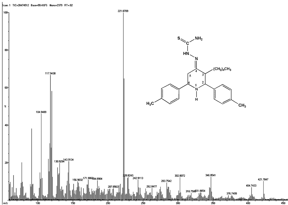
Figure 25. Mass Spectrum of 7
