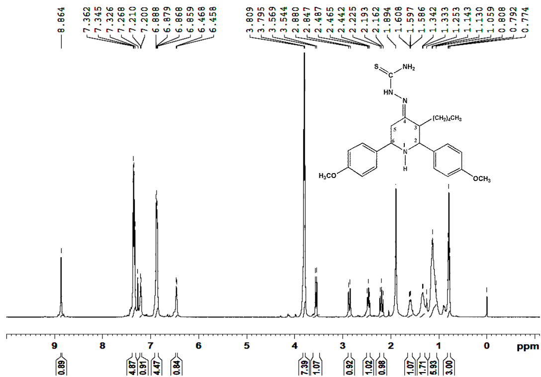
Figure 17. ^1\text{H} NMR Spectrum of 5 in \text{CDCl}_3
