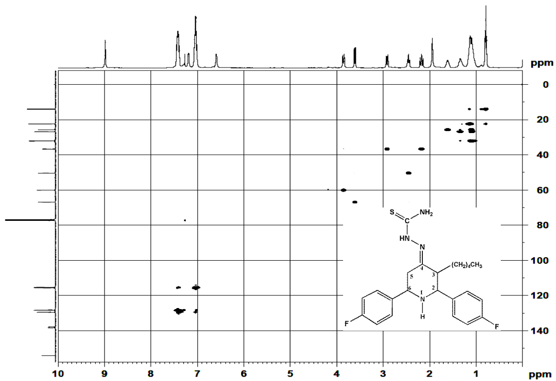
Figure 7. HSQC spectrum of 2 in CDCl 3
