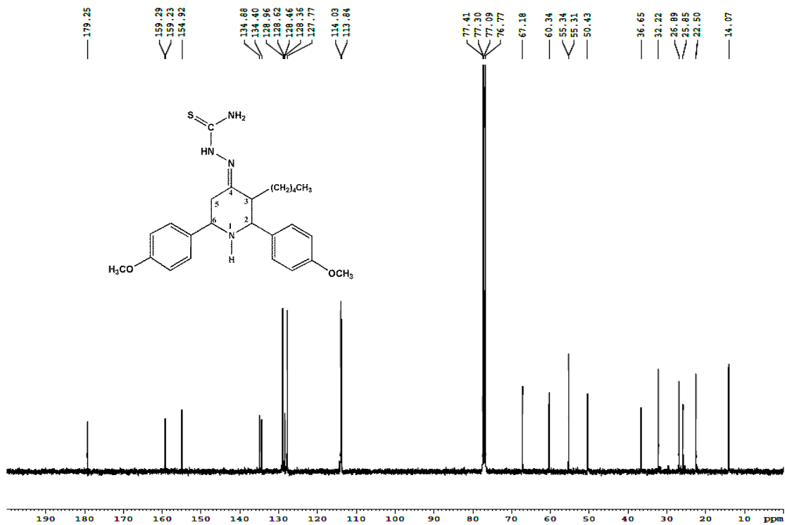
Figure 18. ^{13}\text{C} NMR Spectrum of 5 in \text{CDCl}_3
