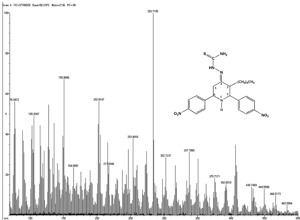
Figure 16. Mass Spectrum of 4
