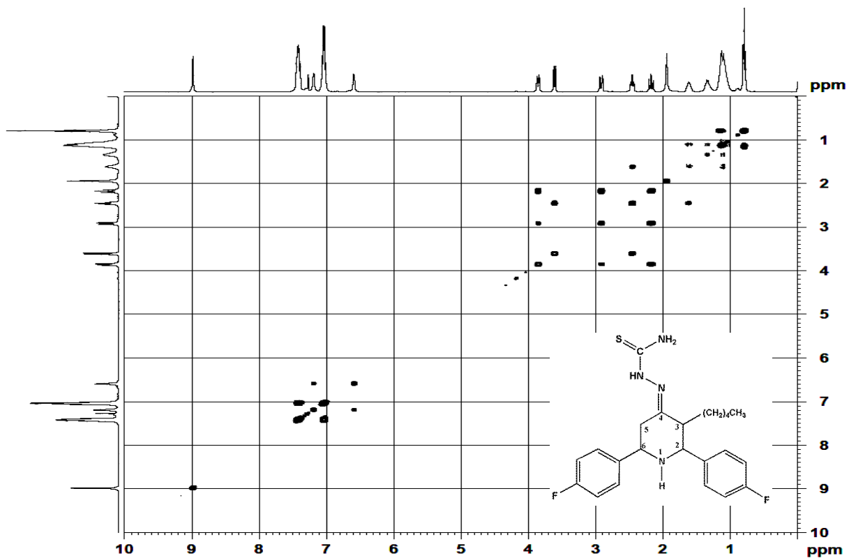
Figure 6. ^1\text{H} - ^1\text{H} COSY spectrum of 2 in \text{CDCl}_3
