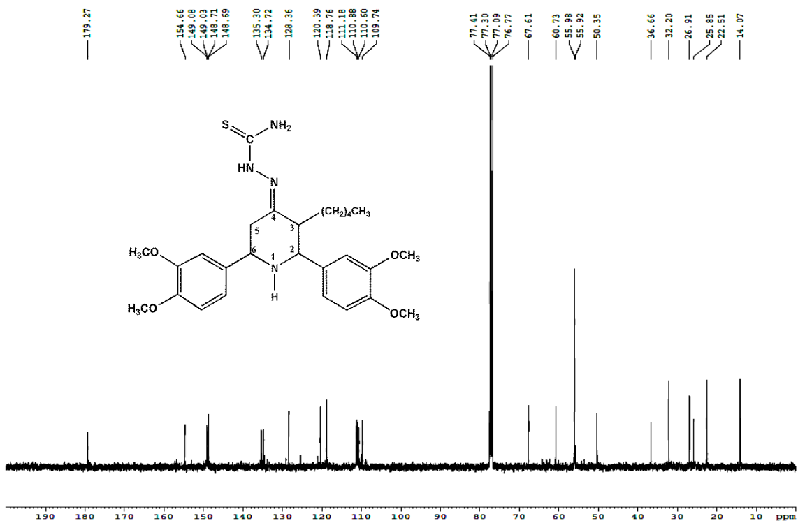
Figure 21. 13 C NMR Spectrum of 6 in CDCl 3
