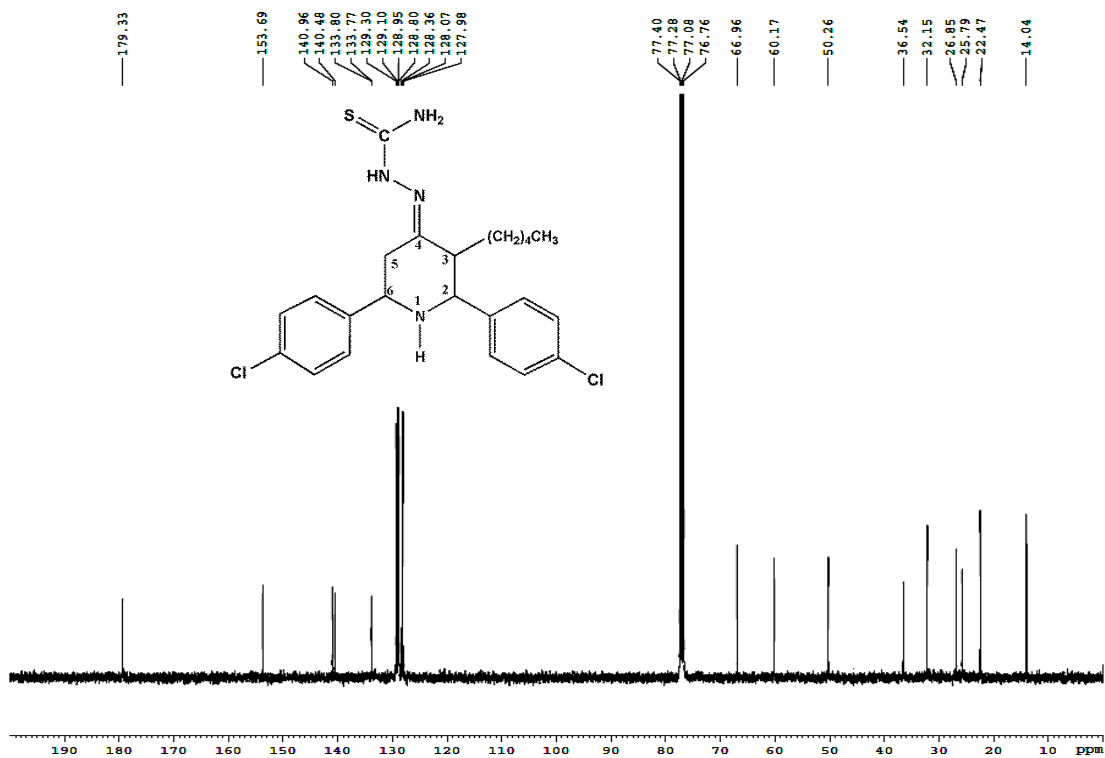
Figure 12. ^{13}\text{C} NMR Spectrum of 3 in \text{CDCl}_3
