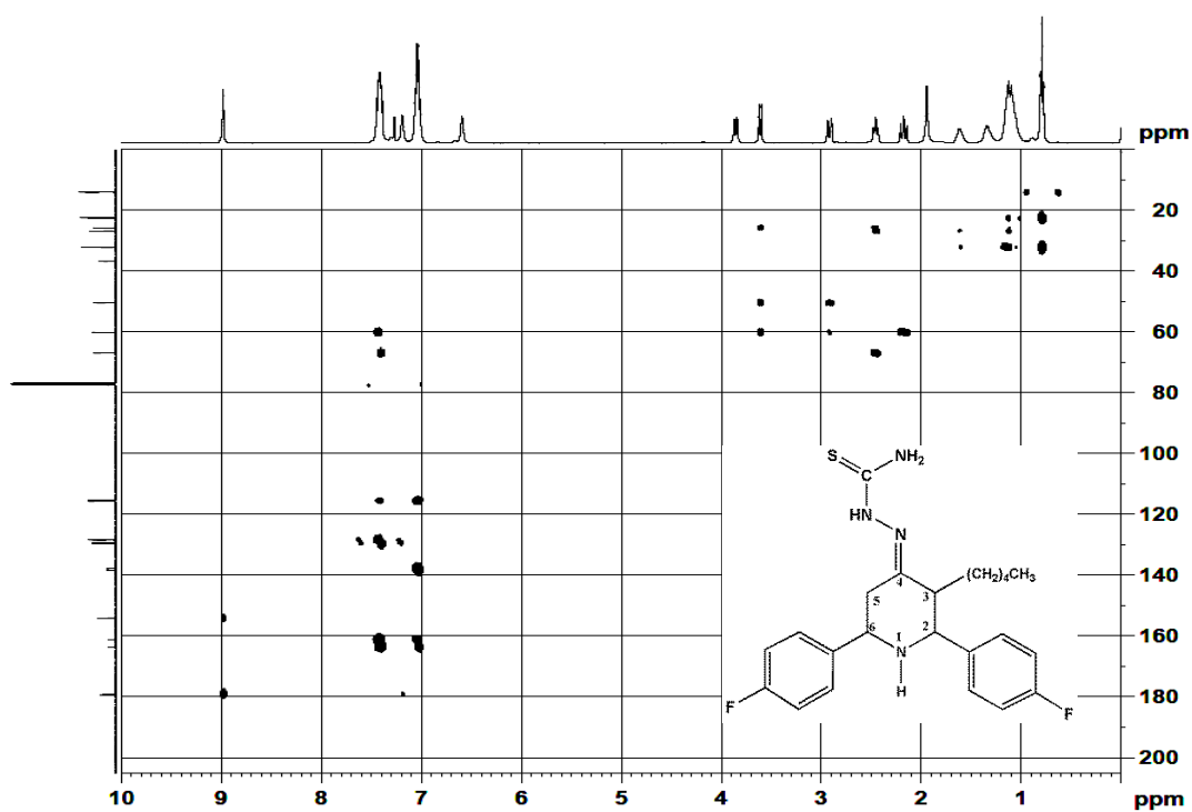
Figure 7. HSQC spectrum of 2 in CDCl 3
