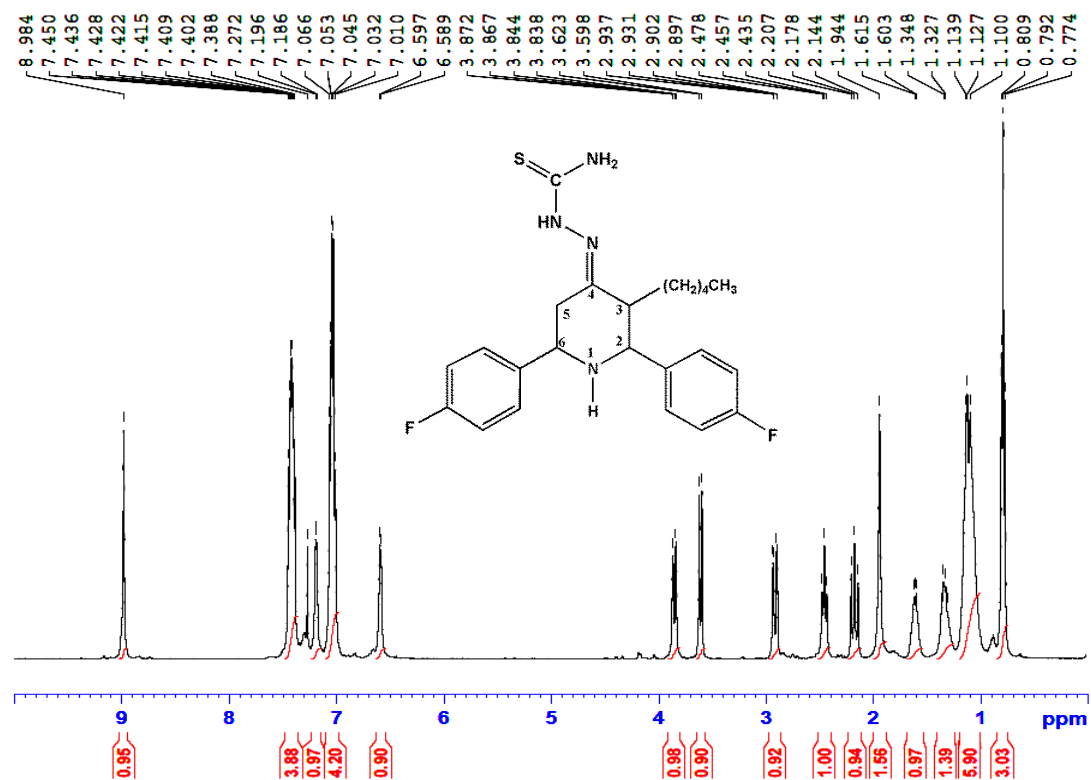
Figure 4. ^1\text{H} NMR Spectrum of 2 in \text{CDCl}_3
