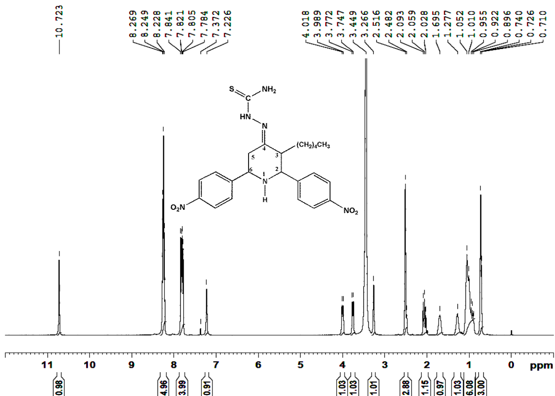
Figure 14. 1 H NMR Spectrum of 4 in DMSO
