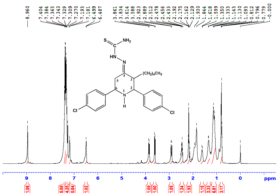
Figure 11. 1 H NMR Spectrum of 3 in CDCl 3
